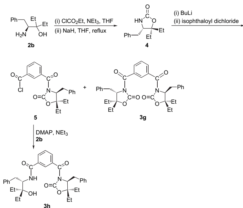
Scheme 2. Synthesis of chiral ligands 3g – h .
