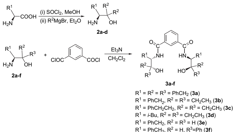
Scheme 1. Synthesis of chiral ligands 3a–f .
